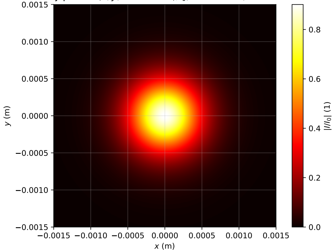
Intensity profile I(x, y, z = 2.149m)/I_0 , Pin=0.6Pcr, artificial time
